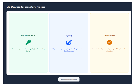
Fig. 14: ML-DSA Process
